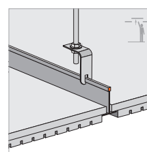
PERFIL SEMIVISTO T-15/T-24 T-15 (9/16") or T-24 (15/16") semi-exposed grid
