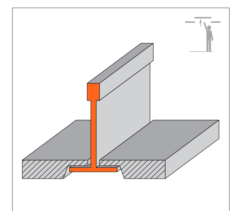
PERFIL SEMIVISTO T-15/T-24 SEMI-EXPOSED FORM T-15/T-24
