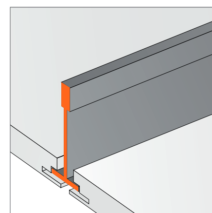
PERFIL OCULTO T-24 RANURA 6 mm CONCEALED FORM T-24 (6 mm)
