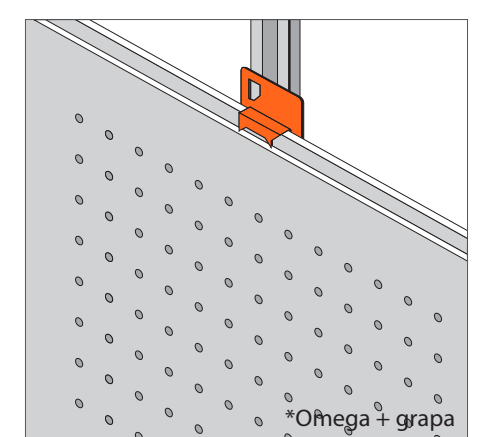
PERFIL MACHIHEMBRADO MALE-FEMALE JOINT *Omega + grapa *Rastrel de madera
