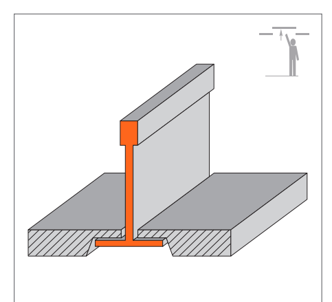
PERFIL SEMIVISTO T-15/T-24 SEMI-EXPOSED FORM T-15/T-24
