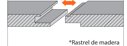
PERFIL MACHIHEBRADO MALE-FEMALE JOINT ■ Omega + grapa ■ Rastrel de madera
