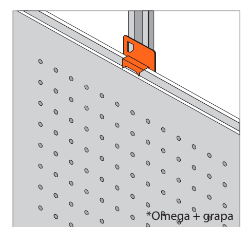
PERFIL MACHIHEBRADO MALE-FEMALE JOINT
