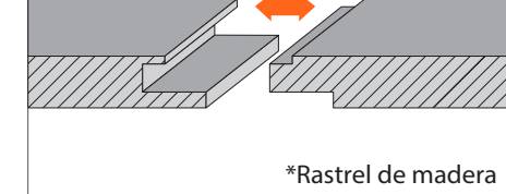
PERFIL MACHICHEBRADO MALE-FEMALE JOINT
