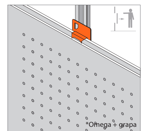
PERFIL MACHICHEBRADO MALE-FEMALE JOINT *Omega + grapa *Rastrel de madera
