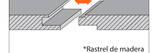
PERFIL MACHICHEBRADO MALE-FEMALE JOINT ■ Omega + grapa ■ Rastrel de madera
