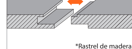
PERFIL MACHIHENBRADO MALE-FEMALE JOINT ■ Omega + grapa ■ Rastrel de madera
