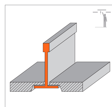
PERFIL SEMIVISTO T-15/T-24 SEMI-EXPOSED FORM T-15/T-24
