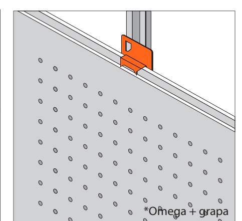
PERFIL MACHICHEBRADO MALE-FEMALE JOINT
