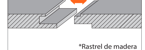
PERFIL MACHICHEBRADO MALE-FEMALE JOINT
