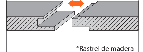
PERFIL MACHICHEBRADO MALE-FEMALE JOINT
