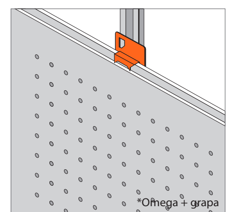
PERFIL MACHICHEBRADO MALE-FEMALE JOINT
