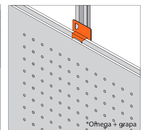
PERFIL MACHIHENBRADO MALE-FEMALE JOINT *Omega + grapa *Rastrel de madera
