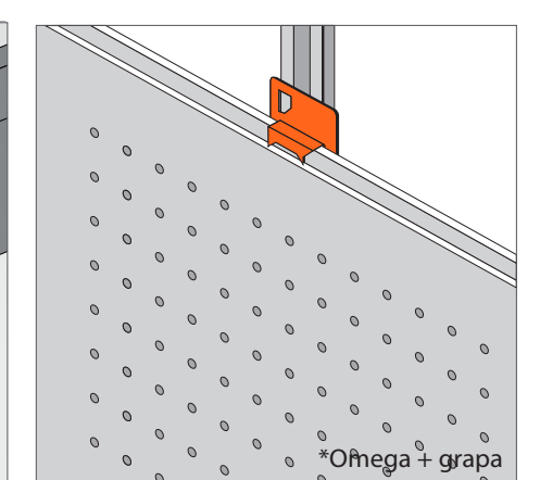
PERFIL MACHIHEBRADO MALE-FEMALE JOINT *Omega + grapa *Rastrel de madera
