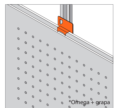
PERFIL MACHICHEBRADO MALE-FEMALE JOINT *Omega + grapa *Rastrel de madera
