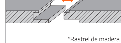
PERFIL MACHIHERRADO MALE-FEMALE JOINT ■ Omega + grapa ■ Rastrel de madera
