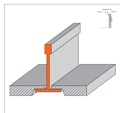
PERFIL SEMIVISO T-15/T-24 SEMI-EXPOSED T-15/T-24
