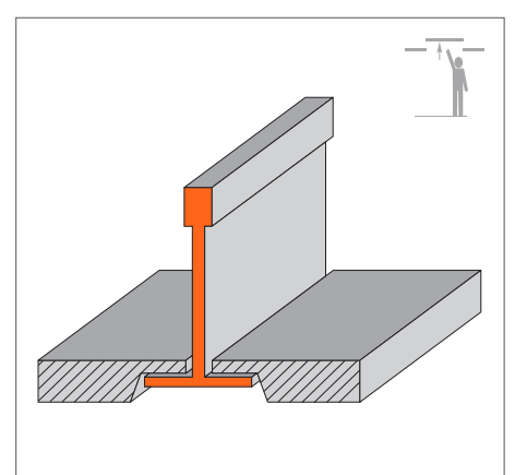
PERFIL SEMIVISO T-15/T-24 SEMI-EXPOSED T-15/T-24
